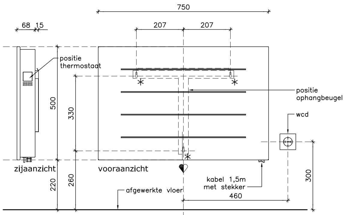
SUBLIME PLUS 500 mm 750 watt - 1.000 watt - 1.200 watt
