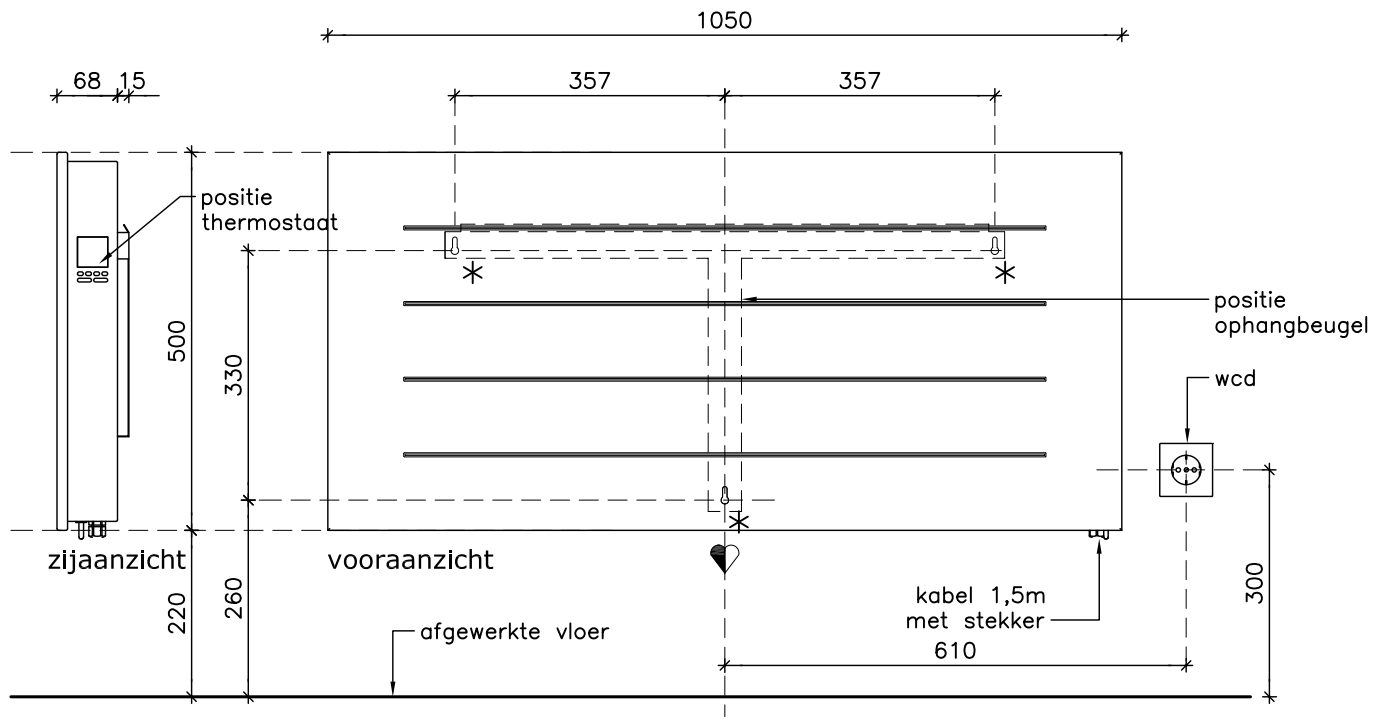
SUBLIME PLUS 500mm 1.500 watt - 2.000 watt
